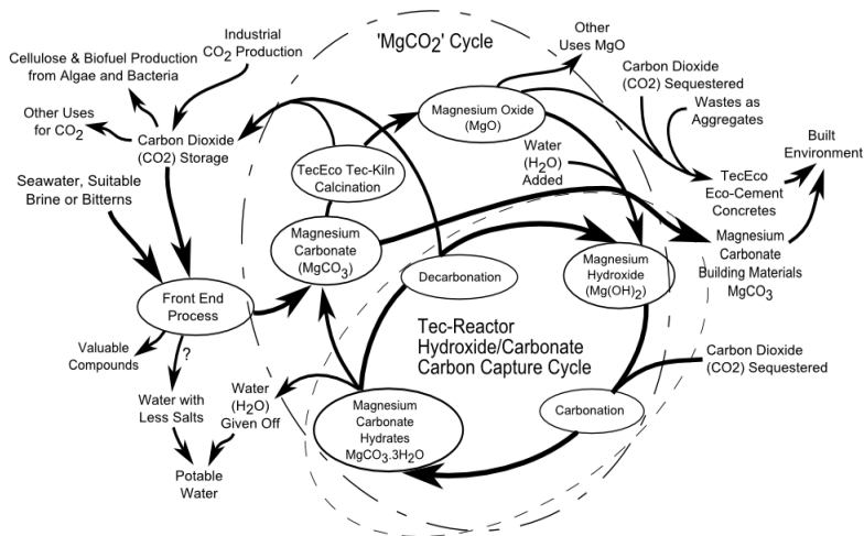
Figure 4 – Gaia Engineering Process Vectors
