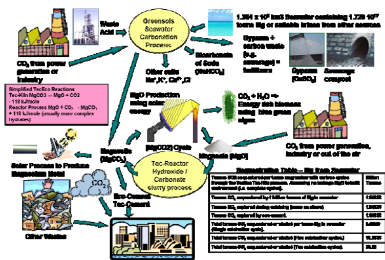
Figure 5 - Gaia Engineering Process Diagram (Greensols Option)
