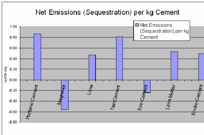
Figure 13 - Net Sequestration Typical Eco-Cement (Assuming Capture during Manufacture)
