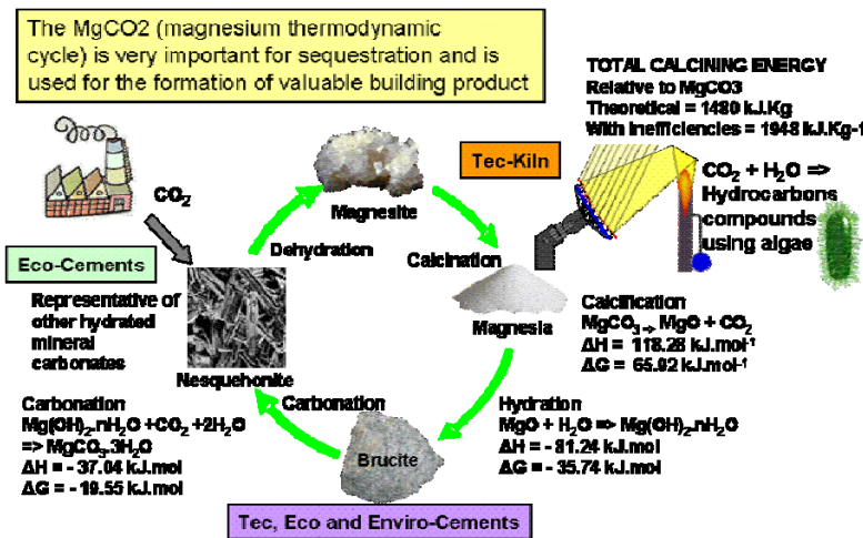
Figure 9 - The Magnesium Thermodynamic Cycle (MgCO 2 cycle)
